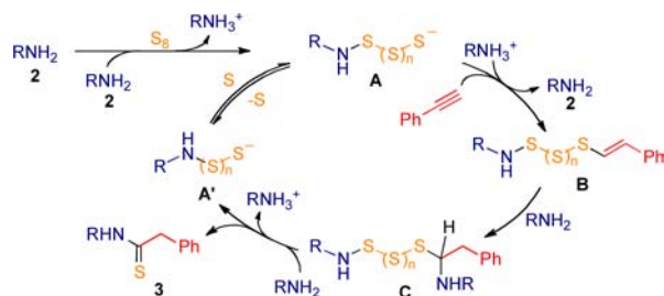
Scheme 3. Proposed Mechanism
