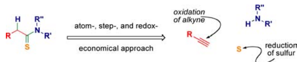
Scheme 1. Atom-, Step-, and Redox-Economical Approach to Thioamide
